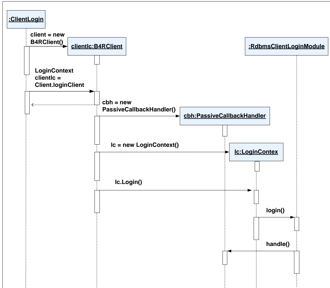
Figure 4.4 – Authentication Sequence Diagram
