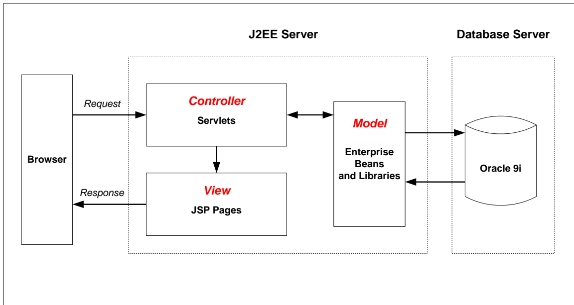
Figure 4.38 – Model-View-Controller architecture
