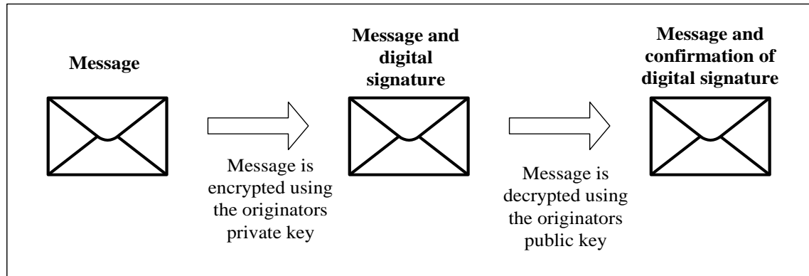
Figure 3.5 – Digital Signature
