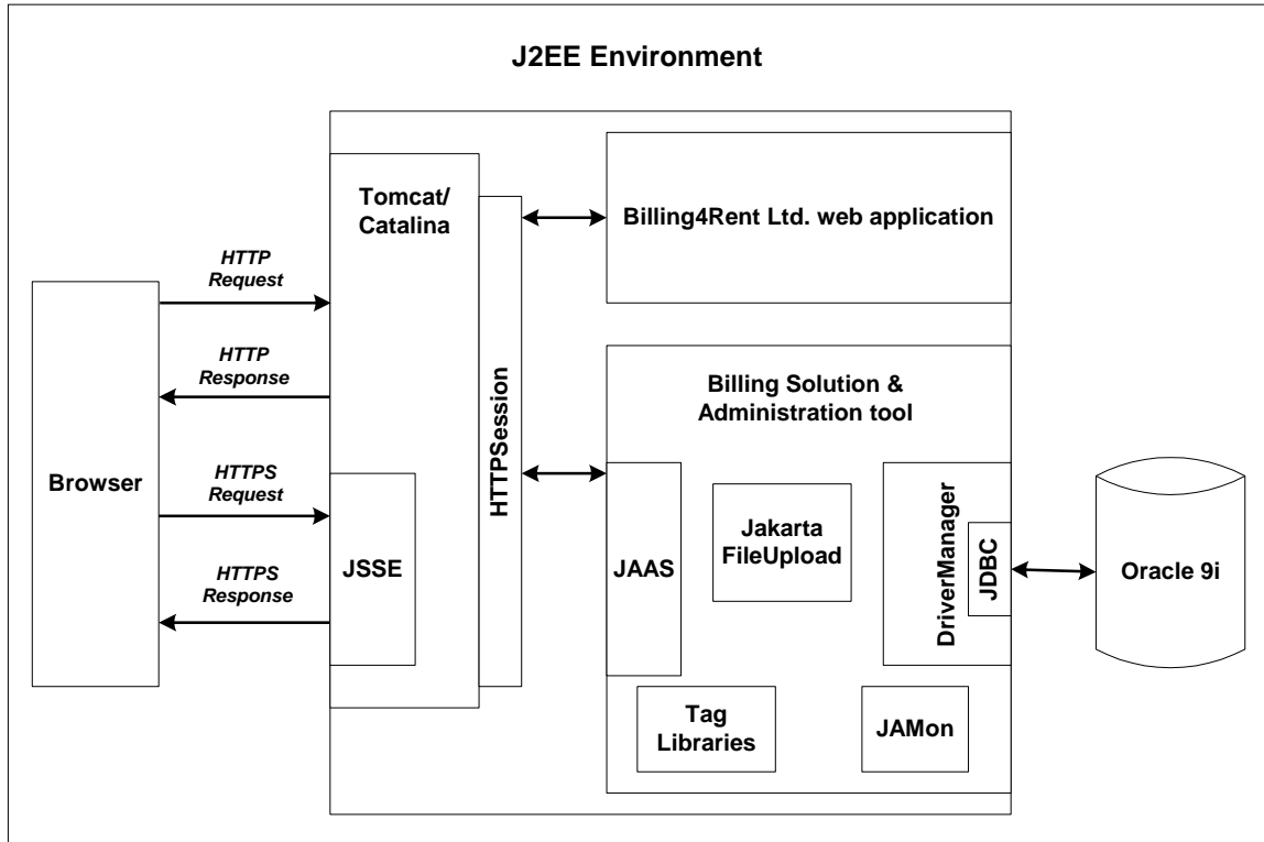
Figure 4.2 – Billing4Rent solution architecture
