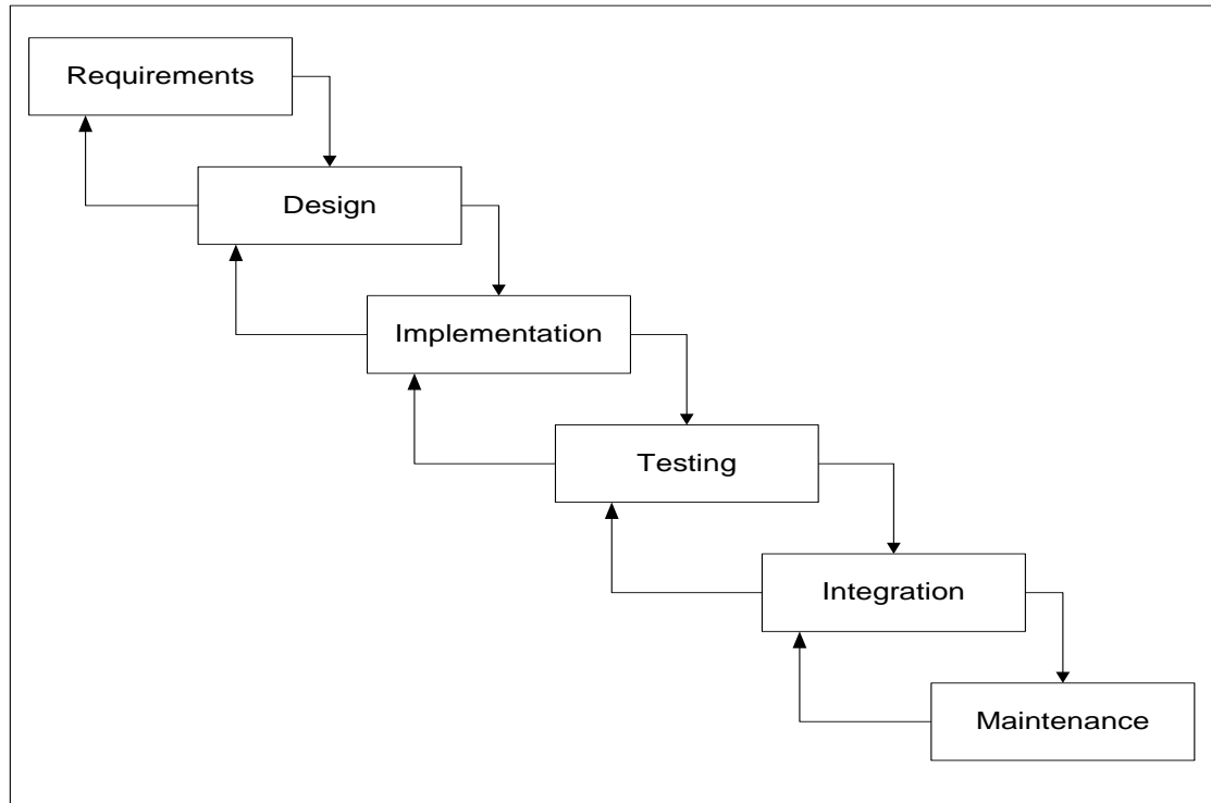
Figure 2.1 – Waterfall Model
