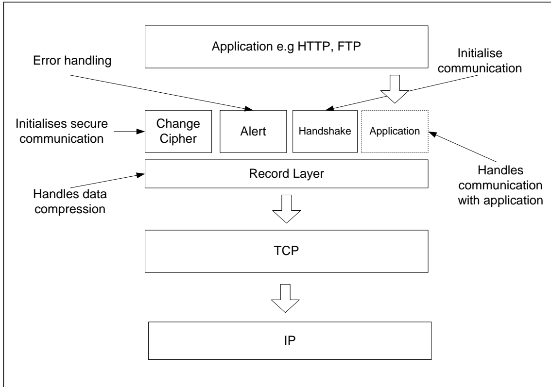
Figure 3.7 – SSL/TLS Protocol
