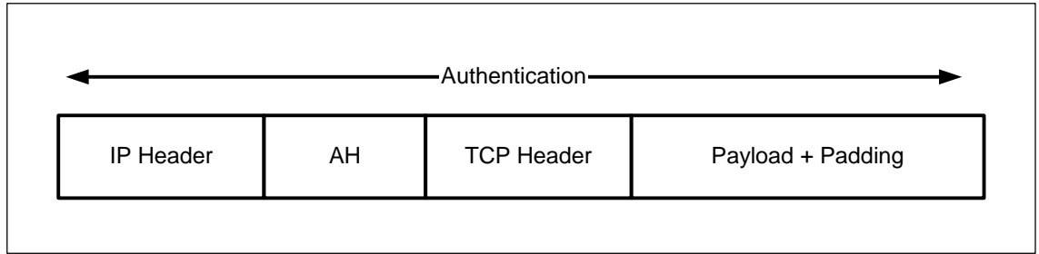
Figure 3.10 – IP AH transport mode
