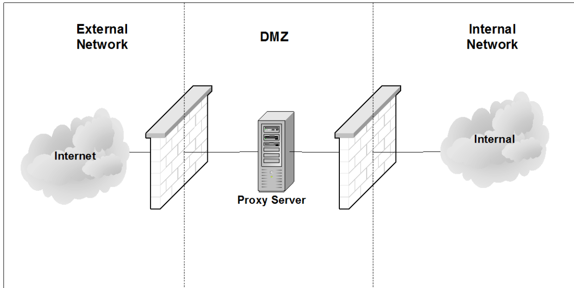
Figure 5.5 – Two-tier, proxy-enabled DMZ design adapted from [109]
